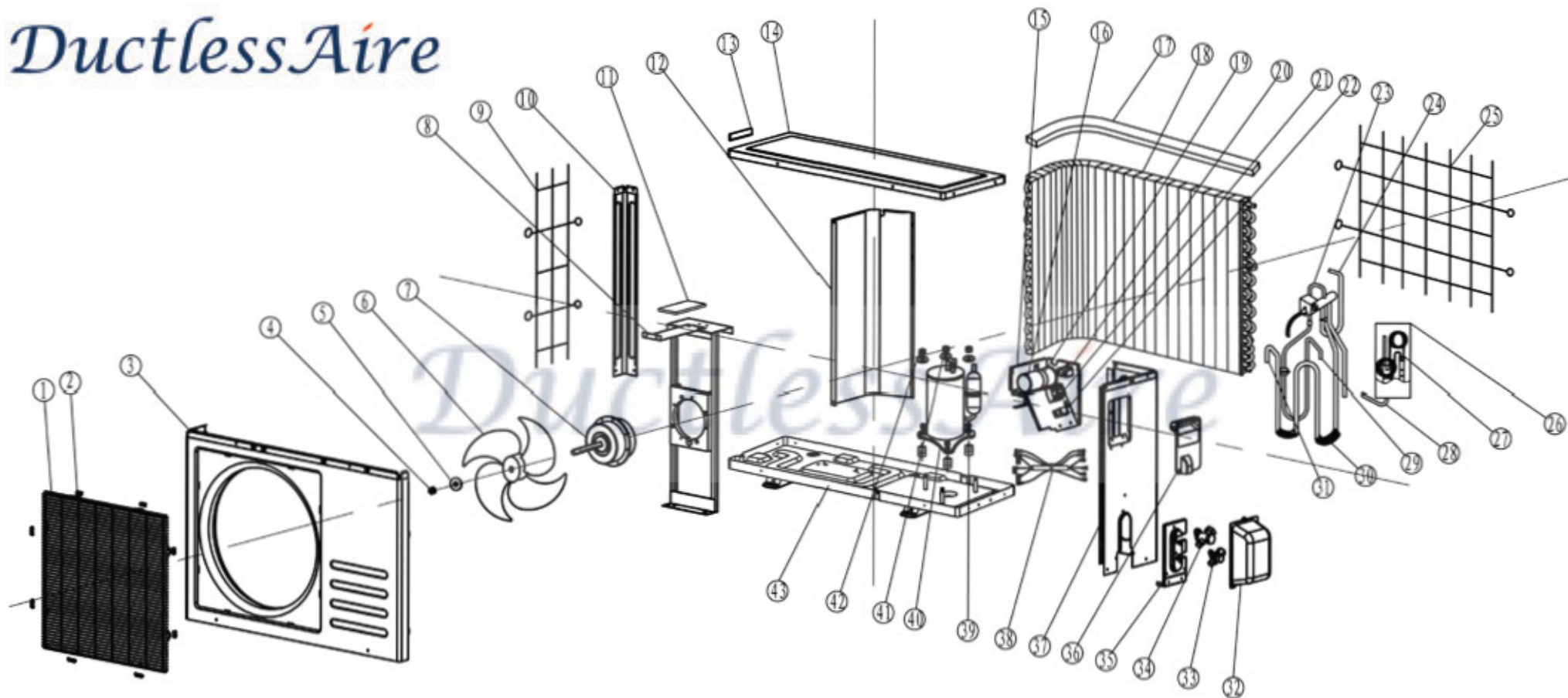
DA1213-H120/O OUTDOOR UNIT EXPLODED VIEW
