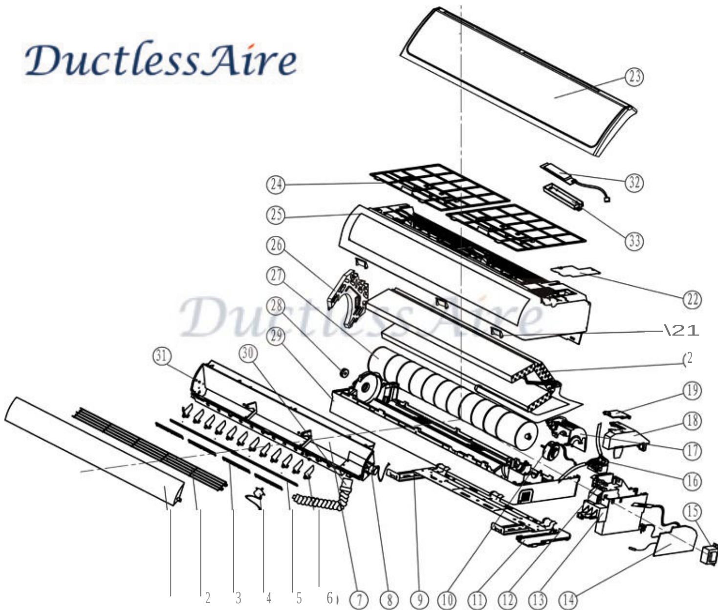
DA1213-H120/INDOOR UNIT EXPLODED VIEW
